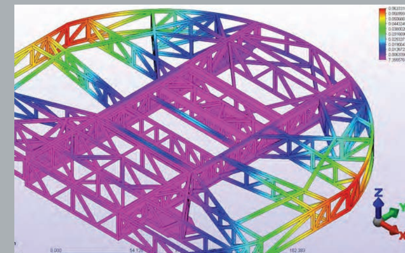
Helicopter Simulator Base
